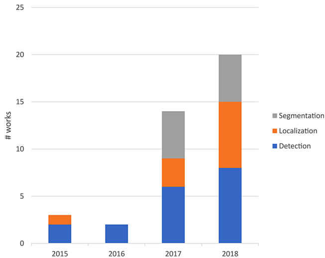
Fig. 2. Literature trends.
